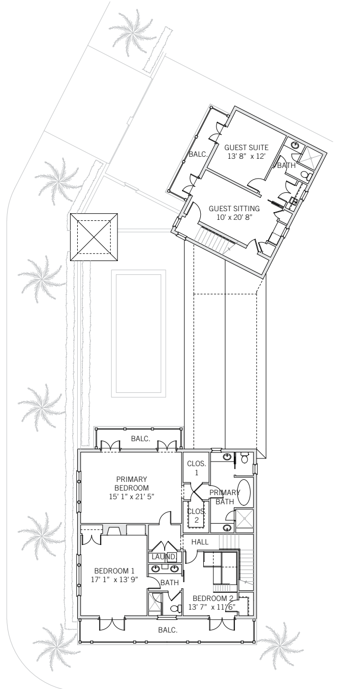
SECOND FLOOR
