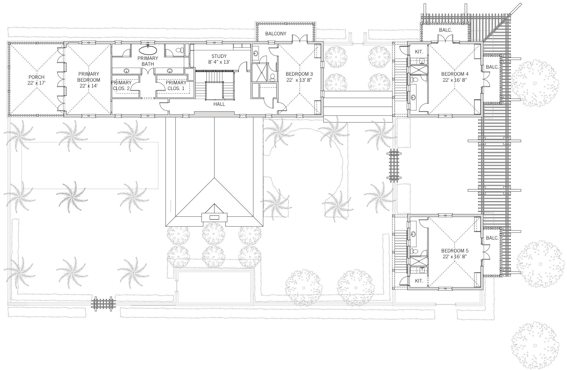
N SECOND FLOOR PLAN
